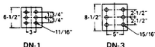
UPPER & LOWER BRACKET DRILLING
