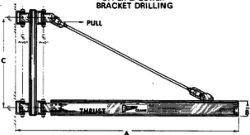
MODEL 360-TDC STANDARD HEADROOM CONSTRUCTION
