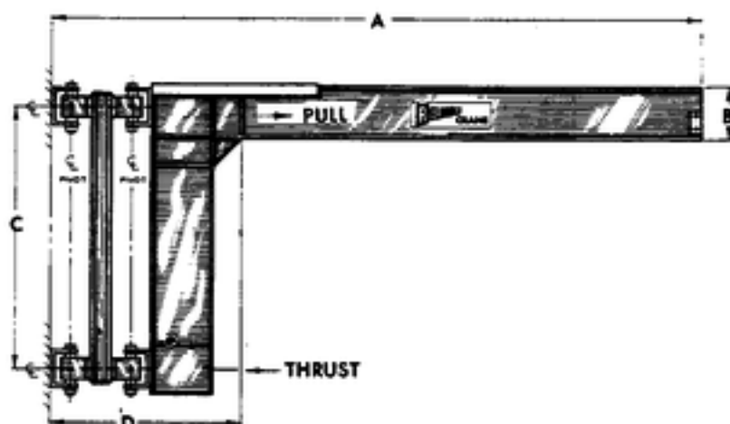
MODEL 360-CDC LOW HEADROOM CONSTRUCTION
